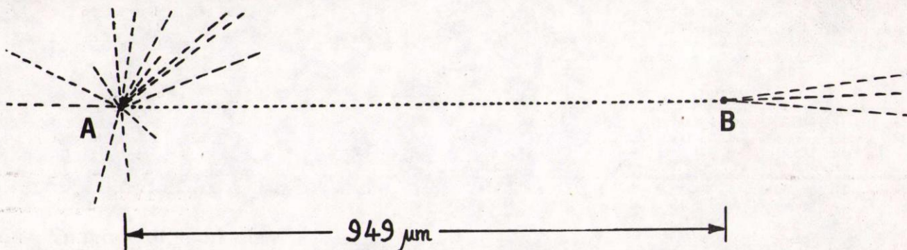
A microphotograph of the decay of a charmed particle observed in an emulsion/bubble chamber experiment at the CERN SPS. A neutrino particle (unseen) enters from the left and interacts at point A, producing a shower of particles. One minimum ionising track (the charm candidate) travels to point B and then decays into 3 charged tracks.
